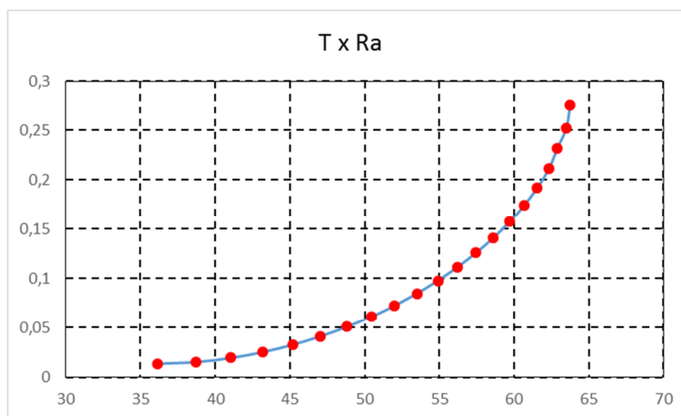
Fig. 2 - Pareto Frontier obtained for NBI method.
