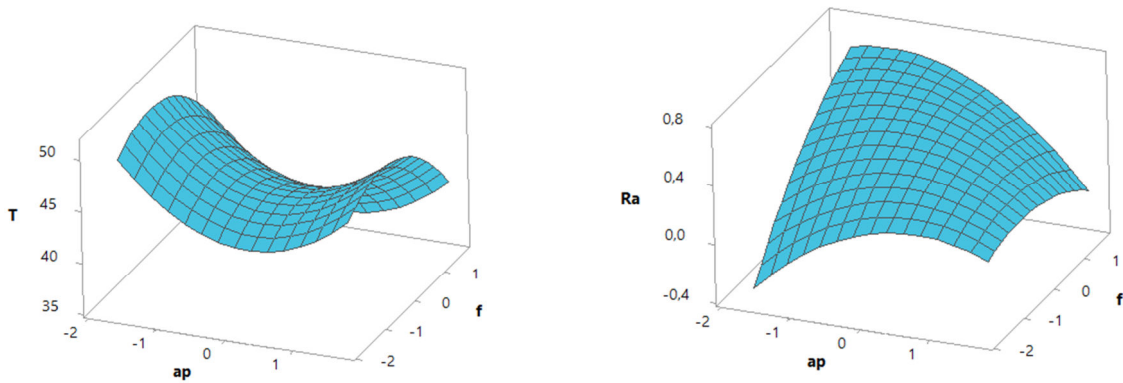
Fig. 1 - Response surfaces for T and Ra.
